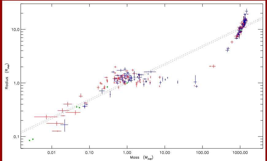
Fig. 1. Plot of the masses and radii of the known transiting planets and their host stars. Blue errorbars show the 58 systems included in the Homogeneous Studies project. Red errorbars show the other 60 transiting systems known as of 2011/04/19. Solar System objects are shown as green circles and the loci of the density of Jupiter and the Sun are traced with grey dotted lines.
