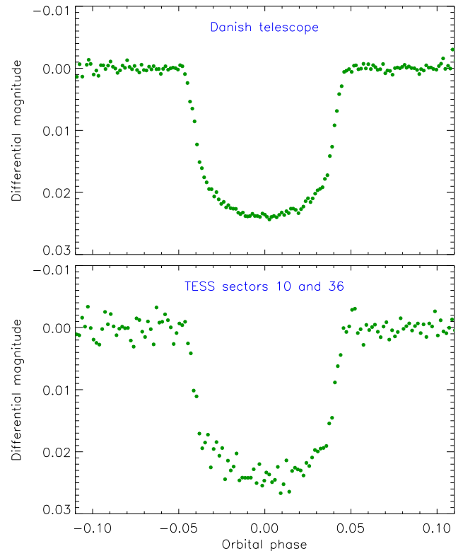
Figure 6. Transit observations of HATS-18 from the Danish Telescope (upper panel) and TESS (lower panel). Each data set has been converted into orbital phase then combined into bins of size 120 s.
