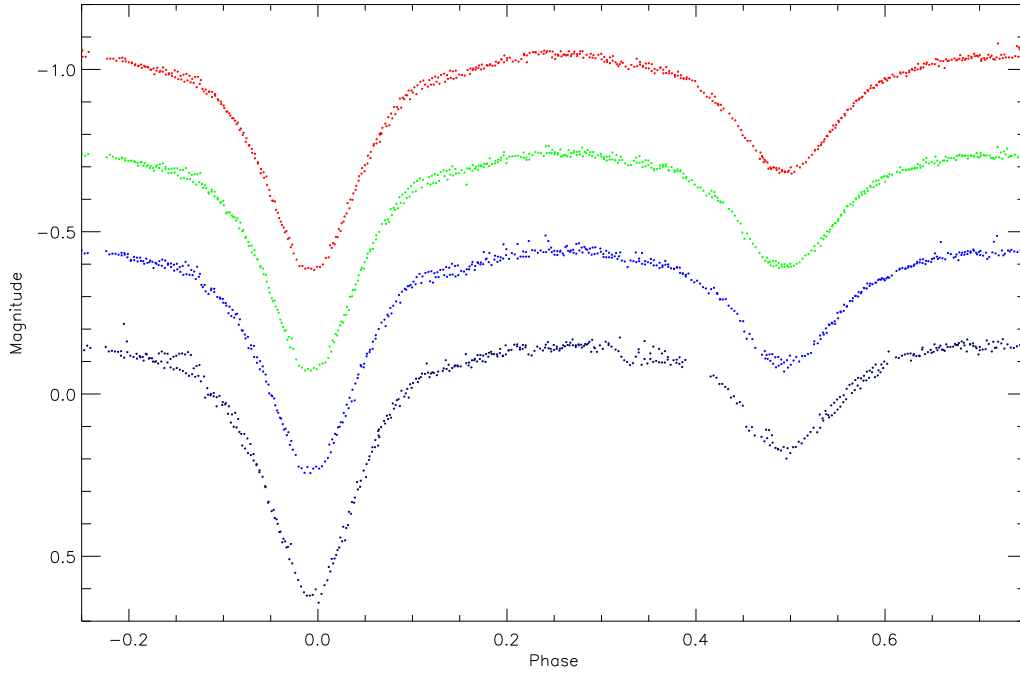
Figure 2. Preliminary (no debiasing or flat-fielding) Strömgren uvby light curve of the eclipsing binary V2263 Cyg in NGC 7128 ( y is at the top and u at the bottom). As it is semi-detached it cannot be used to constrain single-star evolutionary theory, but it can provide an accurate distance to the cluster.
