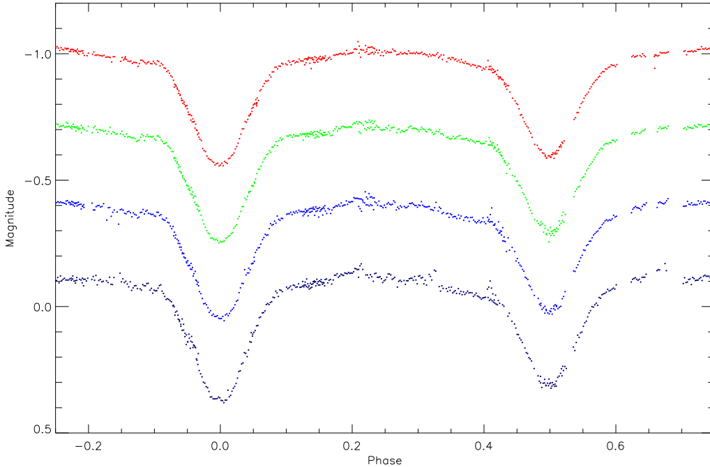
Figure 1. Preliminary (no debiasing or flat-fielding) Strömgren uvby light curves of the detached eclipsing binary V1481 Cyg in NGC 7128 ( y is at the top and u at the bottom).
