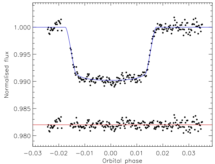
Fig. 1. Phased light curve of WASP-7 compared to the best fit found using JKTEBOP. The residuals of the fits are plotted at the base of the figure, offset from zero.
