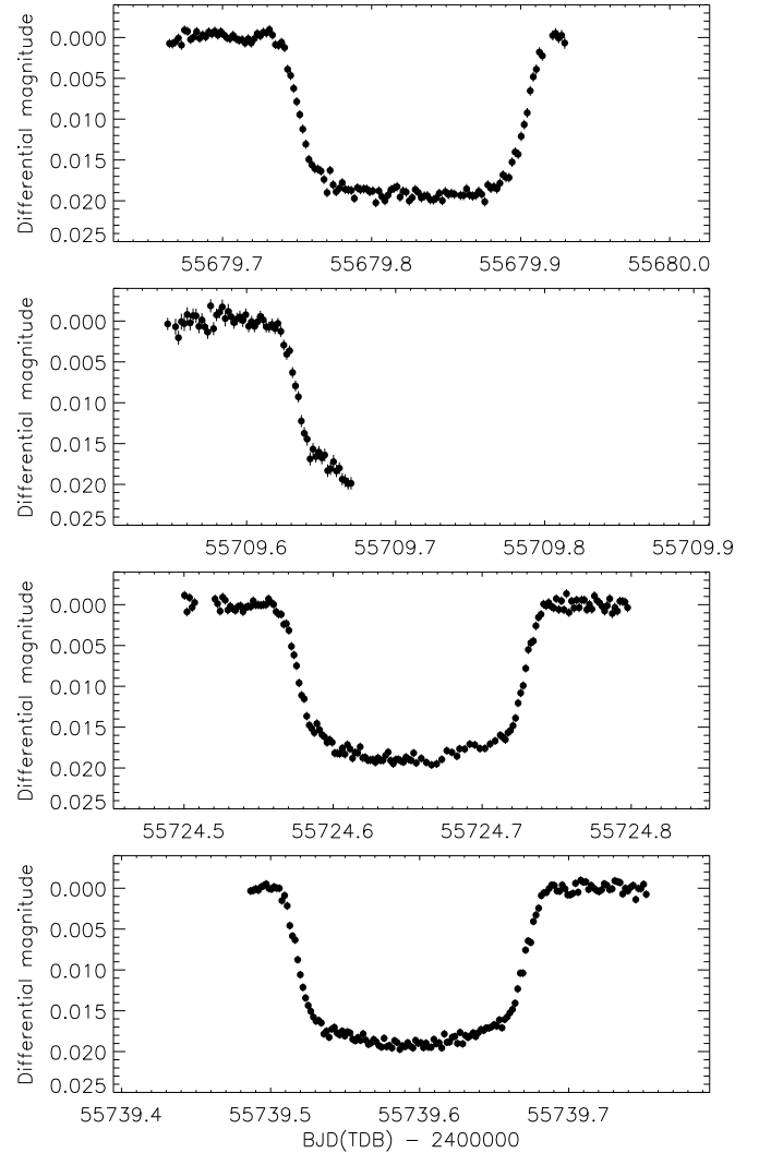
Figure 1. Light curves of WASP-17. The error bars have been scaled to give \chi^2_{\nu} = 1.0 for each night, and in some cases are smaller than the symbol sizes.
