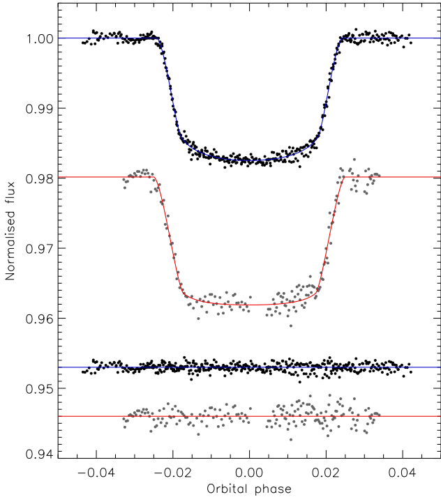
Figure 3. Phased light curves of WASP-17 from the Danish telescope (upper) and the Euler telescope (lower), compared to the best fits found using JKTEBOP and the quadratic LD law. The residuals of the fits are plotted at the bottom of the figure, offset from zero.
