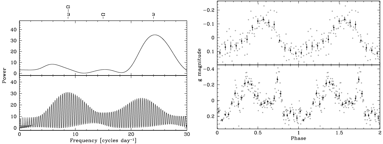
Figure 8. Time series analysis of the LT and INT photometry of SDSS J0233. Upper panels: The Scargle periodogram of the INT data of 2005 January 3. Left: a strong peak is present at 24 \text{ cycle day}^{-1} (60 min). Right: the data folded over that frequency (small points) and binned into 15 points. Lower panels: the Scargle periodogram of the two combined nights of LT data from 2004 August. Left: the strongest signal is found at 8.7 \text{ cycle day}^{-1} (166 min), with a number of aliases spaced by \frac{1}{3} \text{ cycle day}^{-1} . Right: light curves of the original data folded with 8.7 \text{ cycle day}^{-1} (small points) and 25-point phase-binned data (large points).
