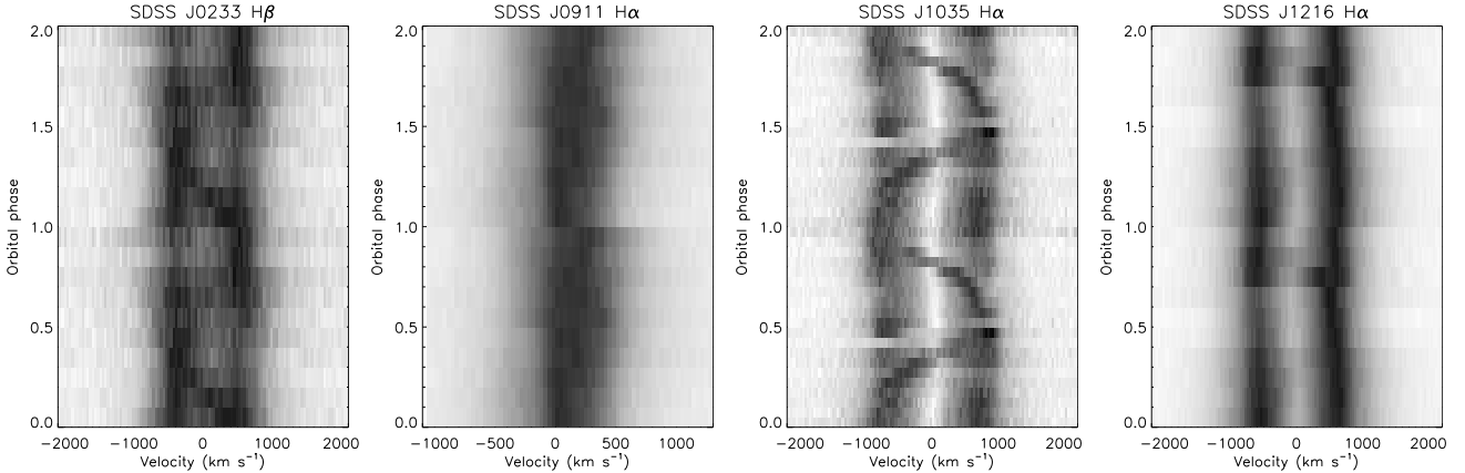
Figure 6. Greyscale plots of the phase-binned trailed spectra of the target CVs.
