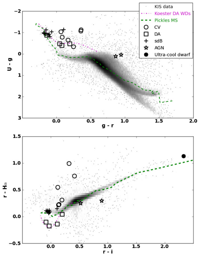
Figure 5. Color-color diagrams of some of the published pulsators, white dwarfs, CVs, ultra-cool dwarfs, and AGNs in the Kepler field. The Pickles tracks are taken from Drew et al. (2005) in the lower panel and from Groot et al. (2009) in the top panel. The magenta tracks in both panels correspond to Koester models of DA WDs with constant surface gravity, \log g = 8 , taken from Verbeek et al. (2012). The gray scale and black points are stellar objects taken from the KIS catalog which have photometric errors smaller than 0.02 mag in all five filters, as well as r -band magnitudes between 12 and 20th mag. The gray scale shows the densest region of the color-color diagrams using a logarithmic scale.
