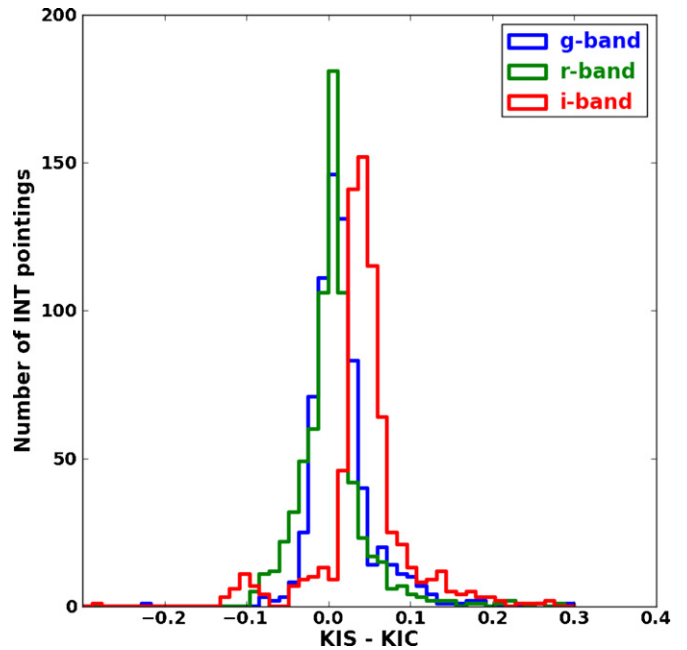
Figure 4. Distribution of \Delta g , \Delta r , and \Delta i , for all pointings, where \Delta\{\text{filter}\} is the offset between the KIC and KIS magnitudes (see Section 3). As one can see, the offsets rarely exceed 5%, and fields with offsets > 0.2 mag from the median are rejected.
