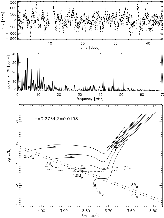
Figure 2. Top: flux as a function of time, after removing the binary signature as described in the text. Centre: the power spectrum of the red giant oscillations. The power excess due to solar-like oscillations is present in the range 30–60 \mu\text{Hz} . The excess below 20 \mu\text{Hz} might be due to granulation in the primary’s atmosphere. Bottom: H-R diagram with BASTI (Pietrinferni et al. 2004) evolutionary tracks for different masses and solar metallicity. The filled circle shows the position of the red giant. The shaded area shows the secondary position constrained by two values derived from the light-curve fit: the radius ratio (dashed lines) and the bolometric luminosity ratio (dashed-dotted lines; taking into account the Kepler bandpass). The asterisk indicates the position of the Sun.
