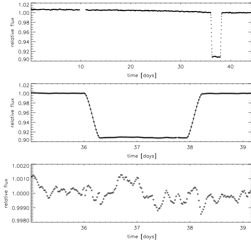
Figure 1. Top: time series data from Kepler of KIC8410637. Middle: a section of the light curve centered on the eclipse with the best-fit model (solid line). Bottom: the residuals after correcting for the eclipse model, clearly showing the solar-like oscillations.
