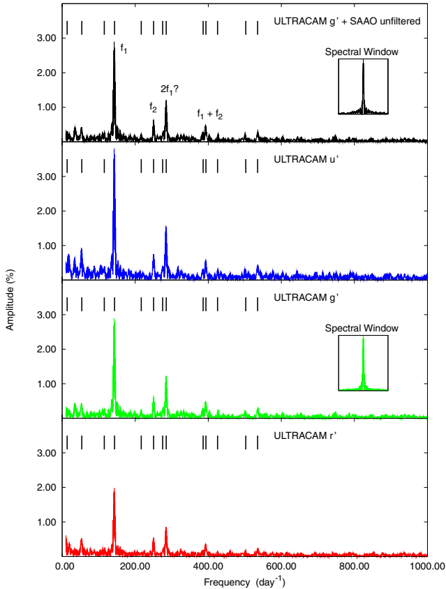
Figure 9. Amplitude spectra for the 2005 May observations of SDSS 1610. The top plot uses the VLT + ULTRACAM g' -band data combined with the SAOA 1.9 m + UCT photometer white-light data. The blue, green and red plots use just the VLT + ULTRACAM u' , g' and r' data, respectively. We mark the signals listed in Table 3, with the longer marks showing the main modes and the possible linear combinations.
