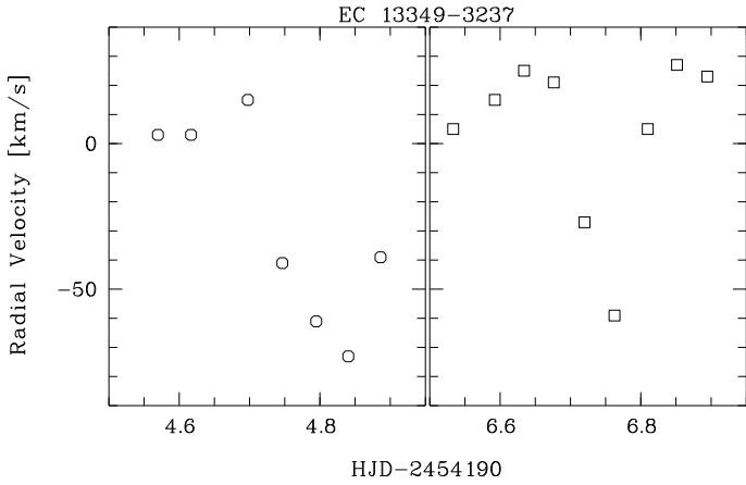
Fig. 11. EC 13349–3237 radial velocities, as determined by a cross-correlation of the absorption forest in-between \lambda 5163\text{--}5338 Å with a synthetic template.
