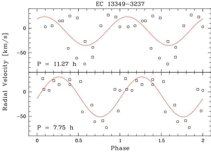
Fig. 10. EC 13349–3237 cross-correlation radial velocities folded on the photometric period ( top ) and on the “spectroscopic” period ( bottom ). Symbols are the same as in Fig. 11. The lines shows the best sinusoidal fit with parameters given in Table 4.
