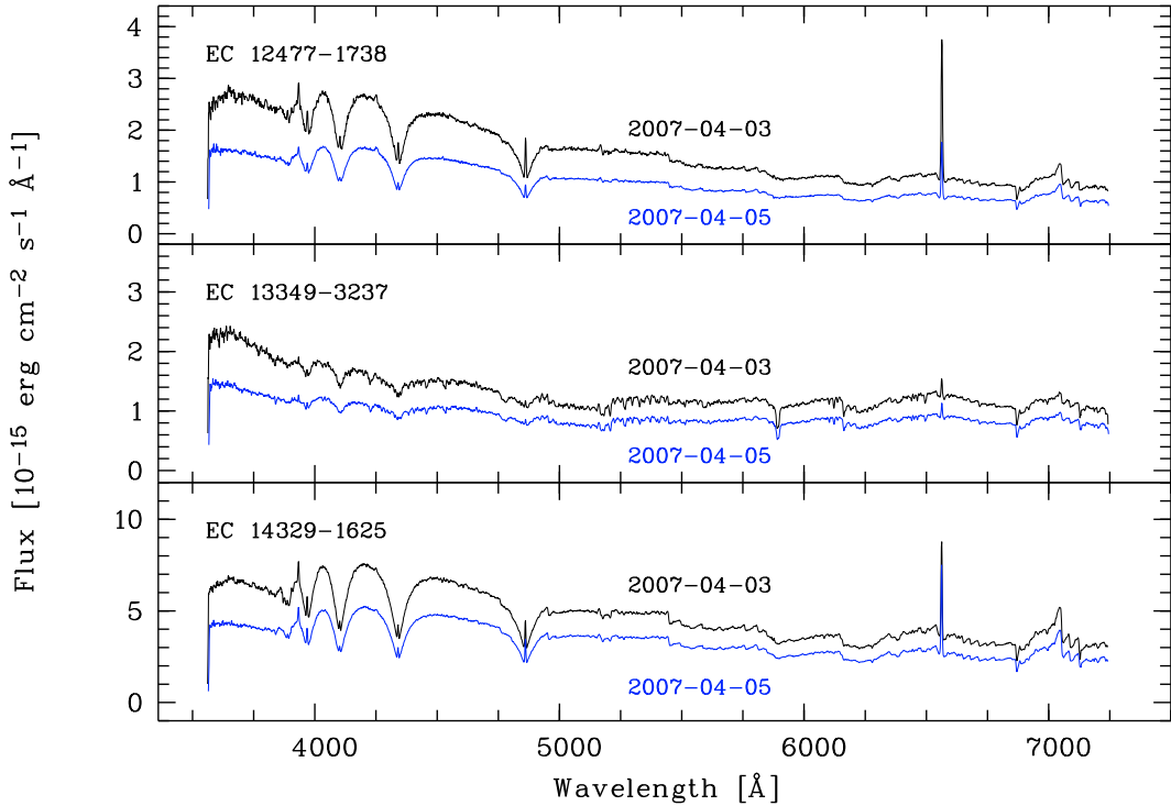
Fig. 2. Average spectra from April 3 and April 5, 2007 as labelled. Note the composite nature of all three systems, with the white dwarf dominating the blue part of the spectrum, and the late-type secondary star showing its presence in the red part. The narrow hydrogen emission lines also originate in the secondary star. The brightness and colour differences between the two nights are not intrinsic. See text for more detail.
